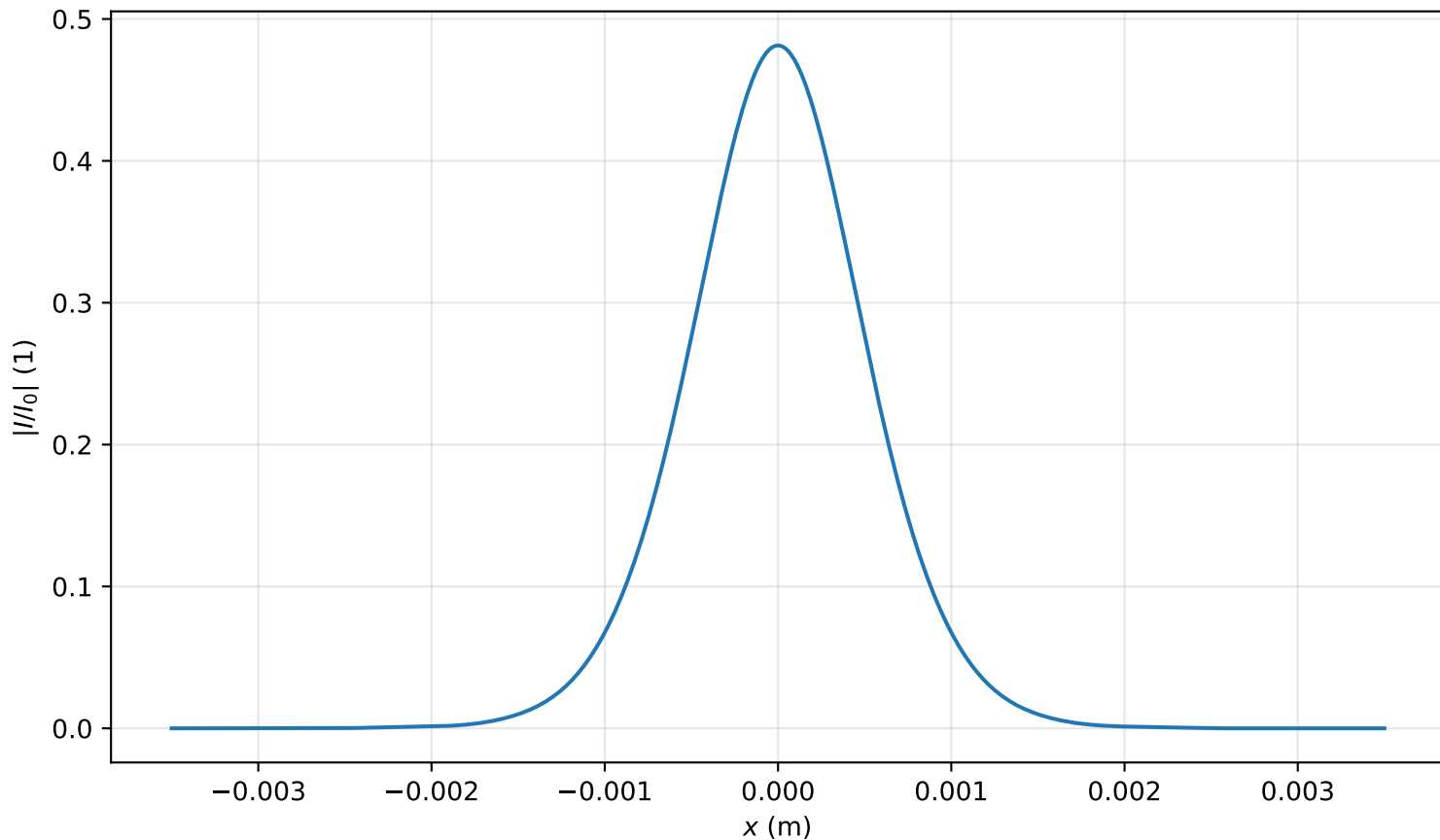
Intensity profile I(x, y = 0, z = 3.423m)/I_0 , P_{in}=0.5P_{cr} , artificial time
